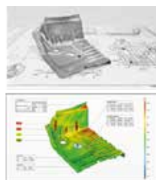
Forming limit diagram before and after tool optimization
